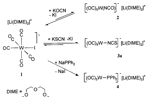
Scheme 1. Substitution of iodide by pseudohalide ions
